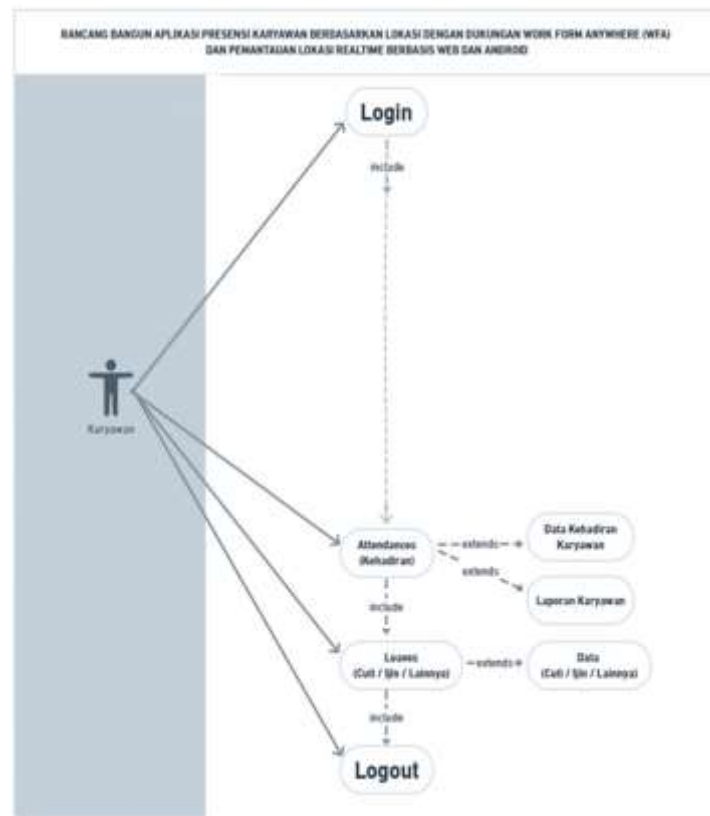
Figure 3. Use Case Diagram (Employee Actor)
